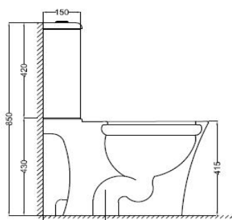
SIDE SECTION
