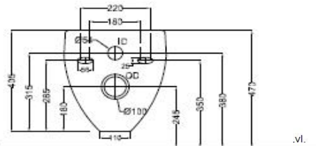
BACK VIEW
